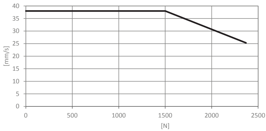
3 x DL6/9/11/16 (equally loaded) with CBD6S (300W)
