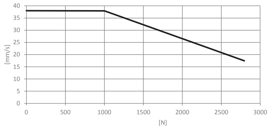
4 x DL6/9/11/16 (equally loaded) with CBD6S (300W)
