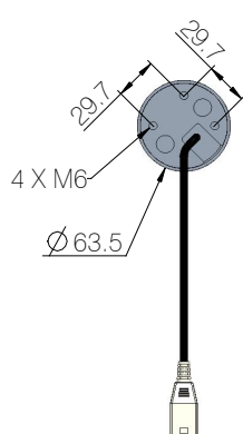
Top plate
