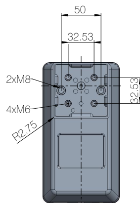
Figure 4 Bottom plate
