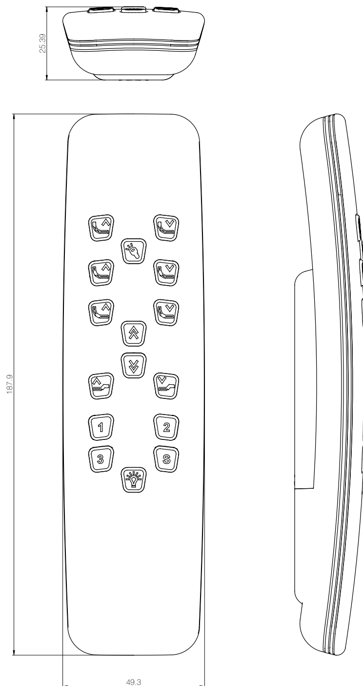
Figure 1 HC20 dimensions
