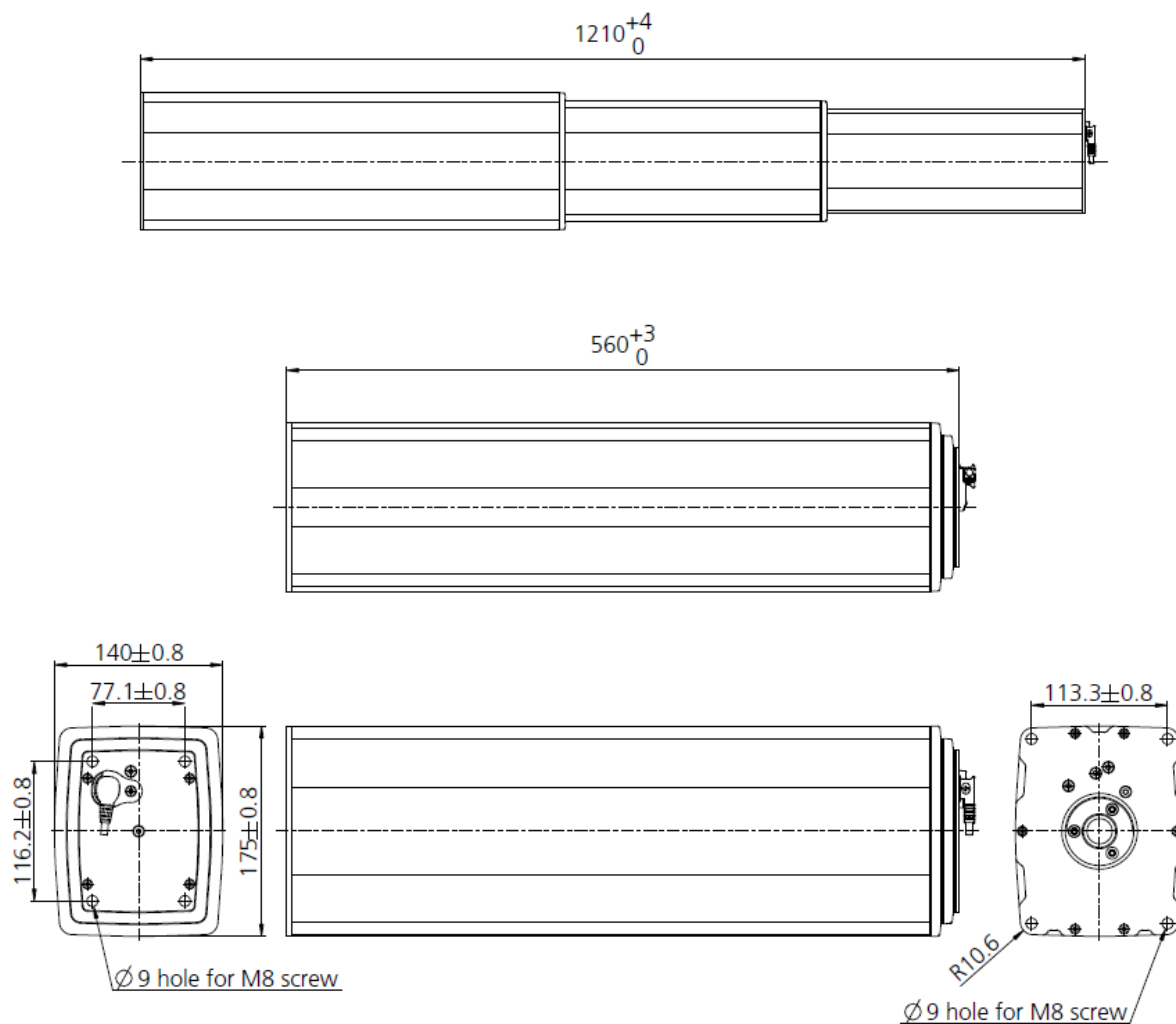
Figure 1 LC1 without end plates dimensions (mm)
