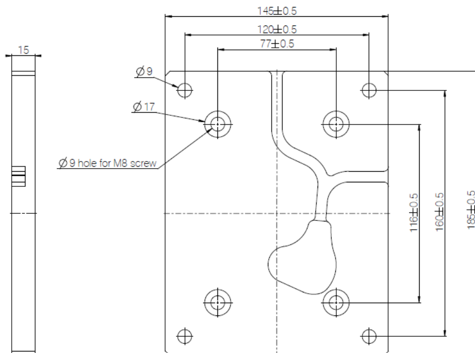
Figure 3 Top end plate dimensions (mm)
