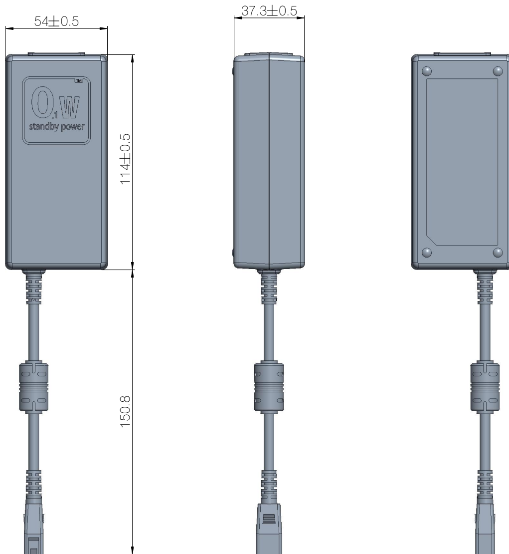
Figure 1 SMPS007 dimensions (mm)
