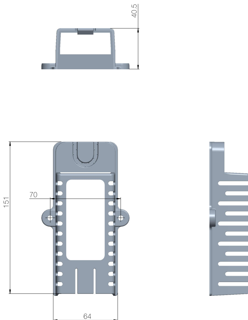
Figure 2 Bracket dimensions (mm)
