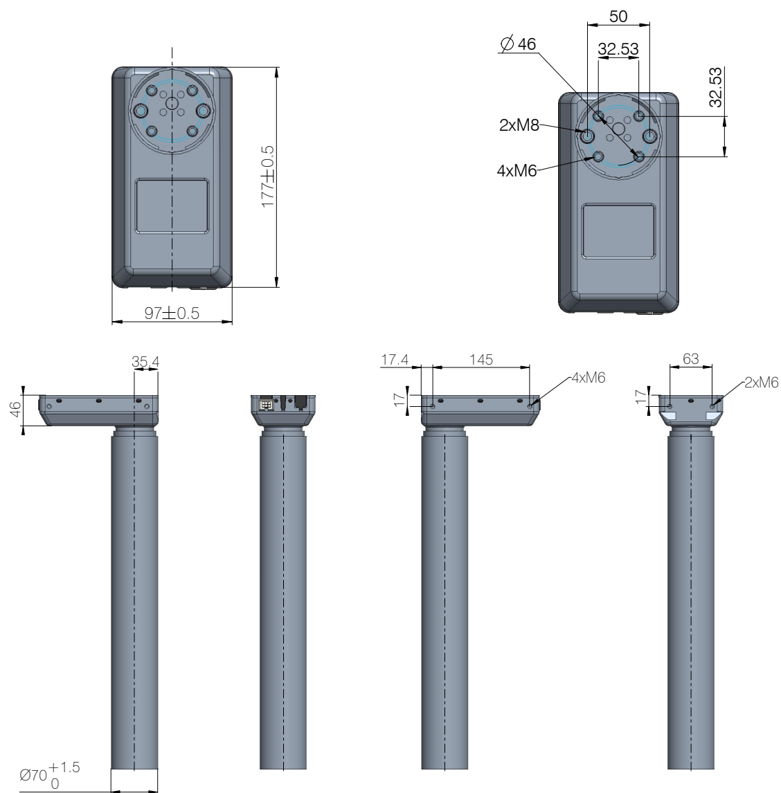
Figure 5 Motor housing, bottom plate, and profile
