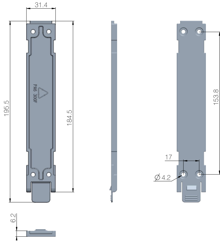
Figure 2 BA001 mounting bracket
