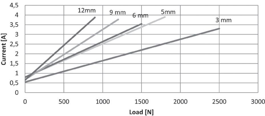
LA23 12V A motor, typical current vs load
