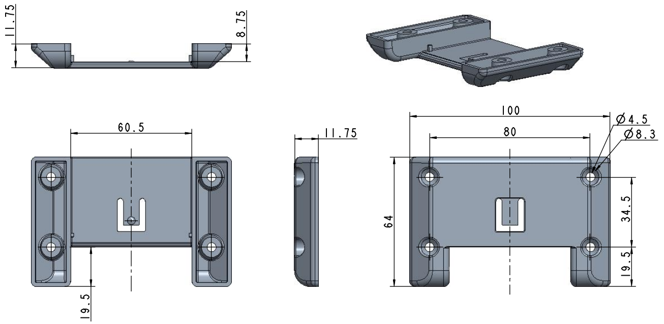
Figure 3 DPB drawer
