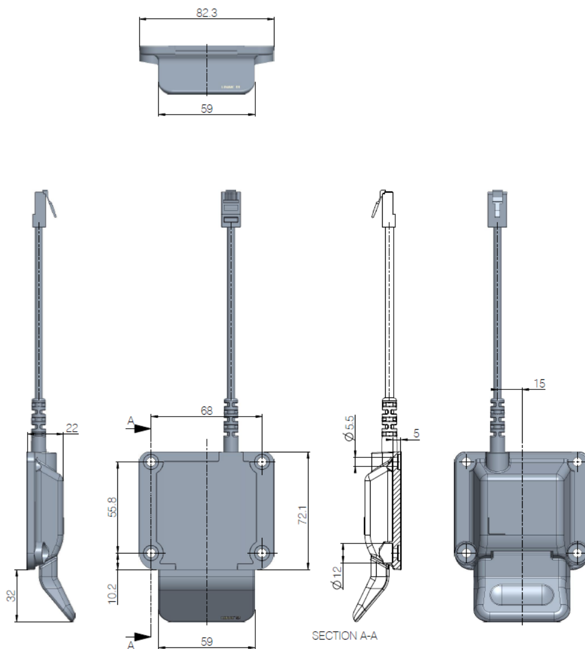
Figure 1 DPI1K dimensions (mm)
