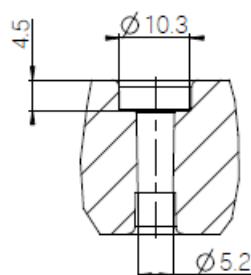
Figure 2 Screw hole
