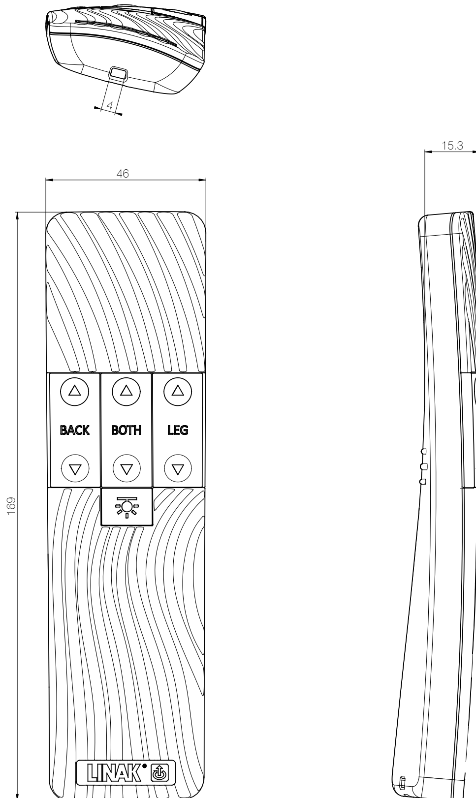
Figure 1 HC40 TWIST™ Standard dimensions (mm)
