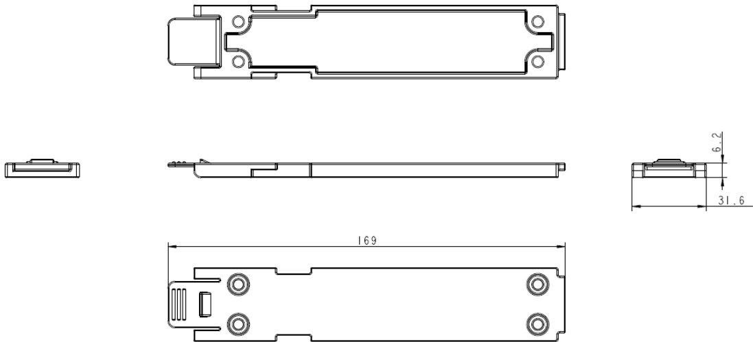
Figure 2 BA002 mounting bracket dimensions (mm)
