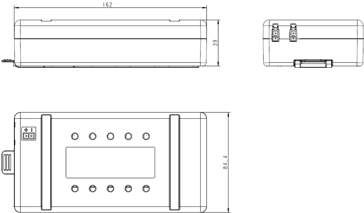
Figure 1 BA002 dimensions (mm)
